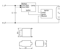
Specificaties Philips SKD 578 220-240V
